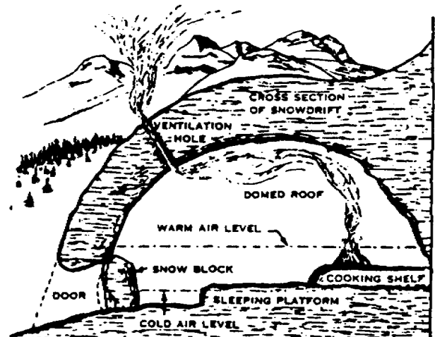
Figure 1-64. Snow cave.
